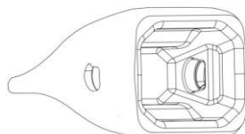
FIG. 27 LEFT REAR VIEW OF AN EXAMPLE EMBODIMENT OF A WEAR MEMBER
