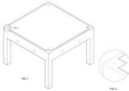
The features of the design for which protection is claimed include the pattern, outline shape and/or configuration and/or ornamentation of a BUILDING MODULE, substantially as shown in the representations.
